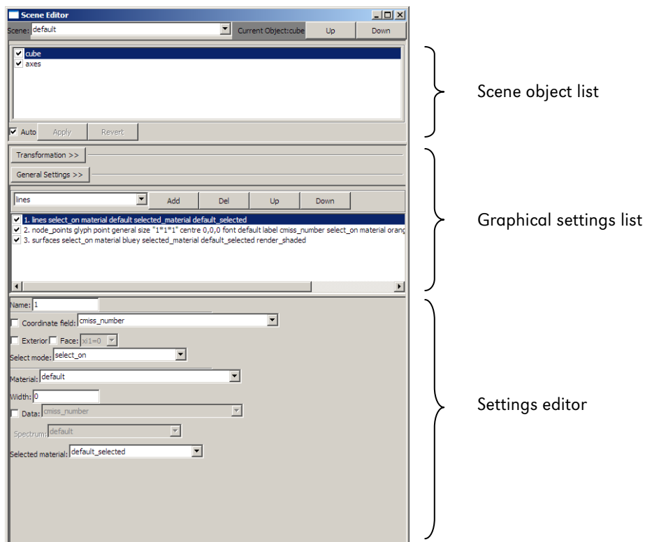
Figure 2: The scene editor window. This window allows you to control the visibility and visual appearance of the objects and graphical settings in a scene.
