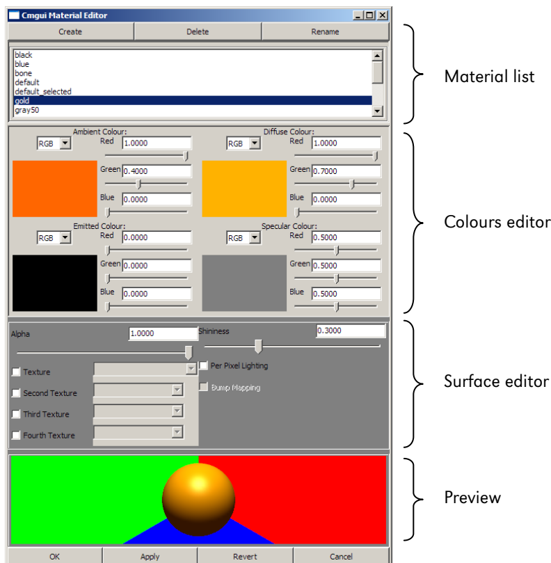
Figure 5: The material editor window
