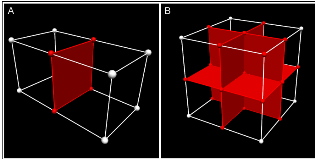
Figure 8: Node, face and line sharing between connected elements In more complex meshes, connected elements share nodes, lines and faces (shared nodes lines and faces are shown in red). In panel A, this two-cube mesh has only 12 nodes; 4 of the nodes are shared by both elements. In panel B, an eight-cube mesh is made up of only 27 nodes - many of the nodes are shared by more than one of the elements. The central node in this example is shared by all 8 elements. Field values are continuous across these shared parts.
